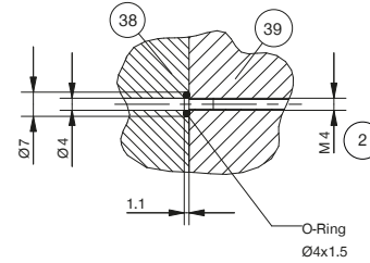
Hoseless air feed-through M4
