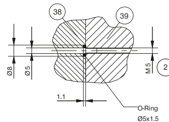
Hoseless air feed-through M5
