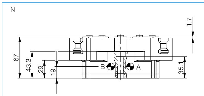
Hoseless air feed-through M5
