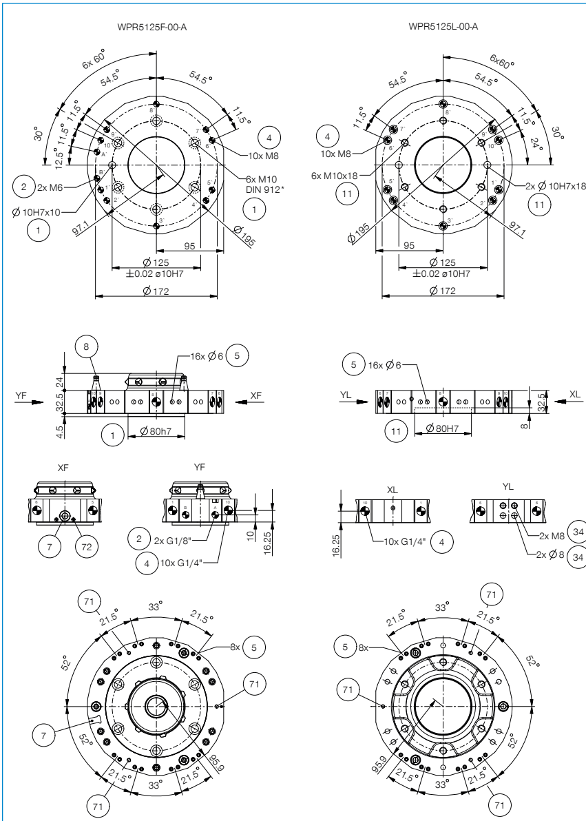
Hostless energy connection (tool side)
