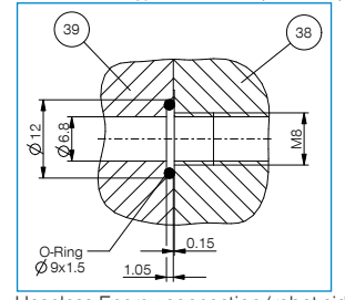
Hoseless Energy connection (robot side)
