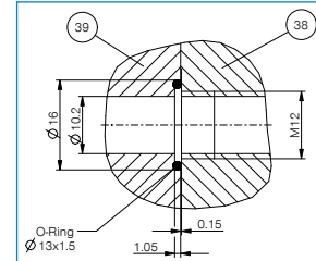
Hoseless Energy connection (robot side)
