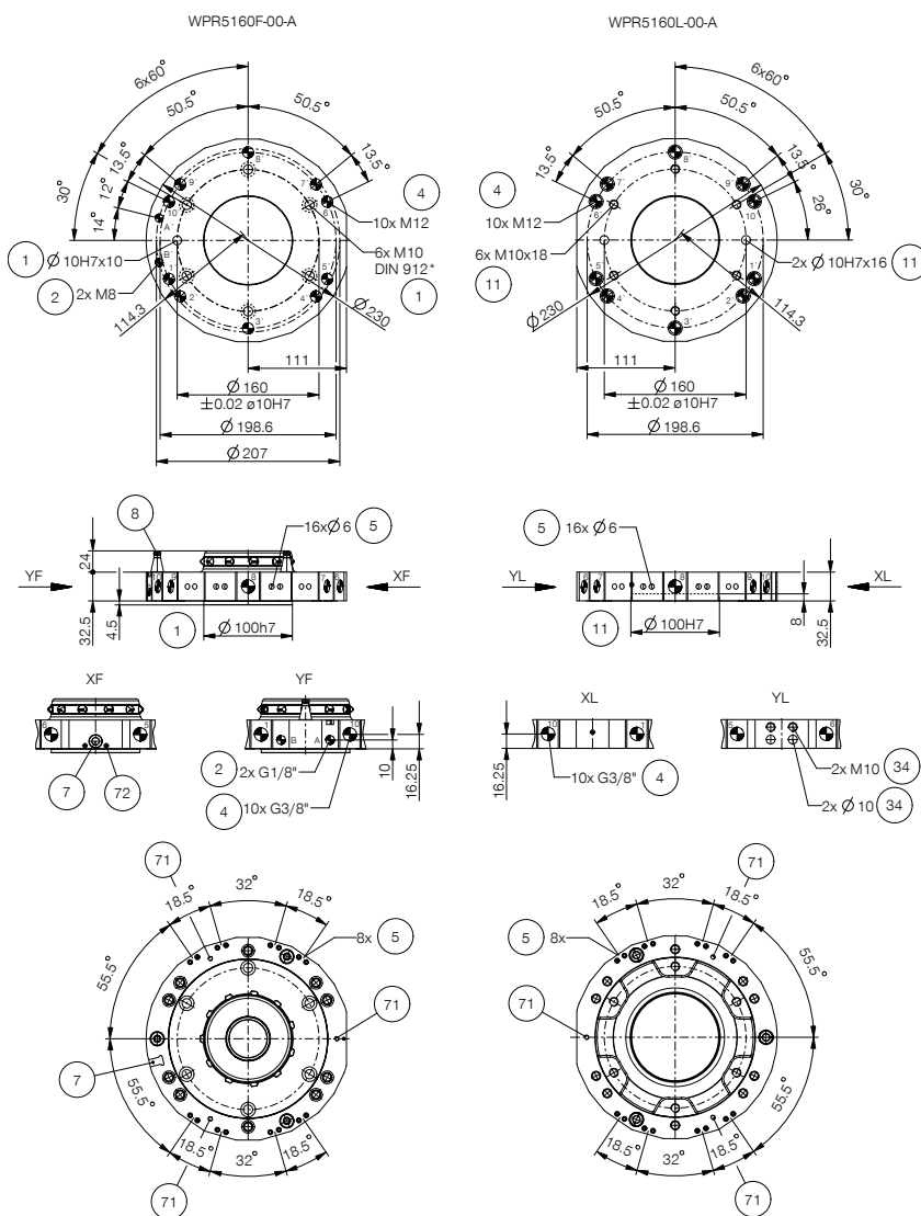
Hostless energy connection (tool side)
