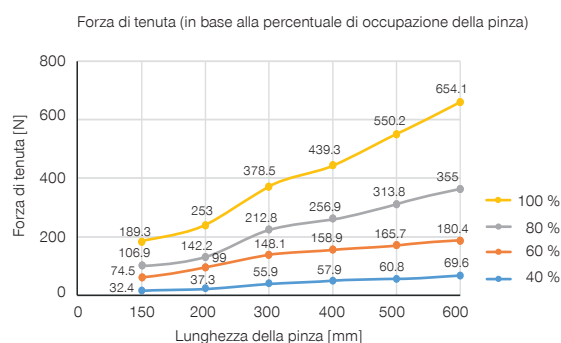
ZGM40 ovale
