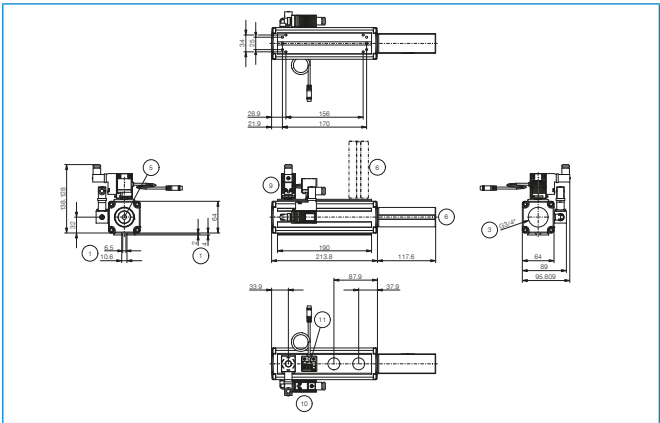
ZMP30304-A-AR3-DL-SN / -SP
