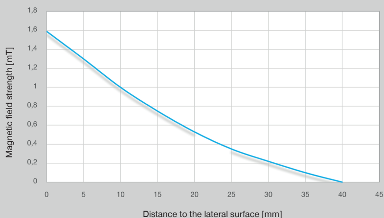
Decrease in the magnetic field over the distance to the lateral surface
