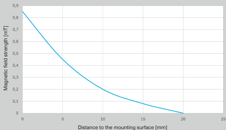
Decrease in the magnetic field over the distance to the mounting surface
